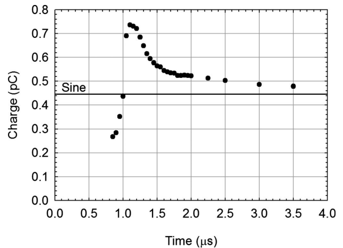
FIG. 9. The on-axis signal as a function of the characteristic FODO waveform rise time \tau shows that for large \tau , where the applied voltage waveform broadly resembles a sinusoid, the measurement is nearly the same as if a true sinusoid had been applied (solid line). As \tau is reduced, the on-axis signal grows until \tau becomes too short, Gibbs ringing in the applied waveform is seen, and the on-axis signal drops sharply.
